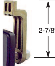
#4 Extra Long Offset Cam Bar as used on 1091/1092 & 1031/1032 for 3/8" Shafts
