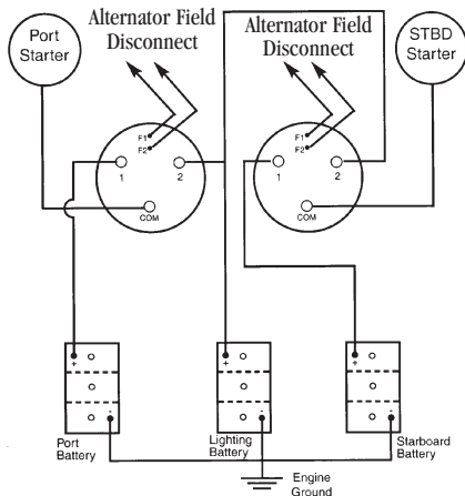
2 ENGINES, 2 ENGINE BATTERIES, 1 SEPARATE BANK OF LIGHTING BATTERIES AND 2 SWITCHES
