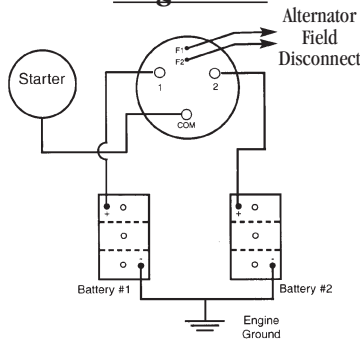
SINGLE ENGINE - TWO BATTERIES
