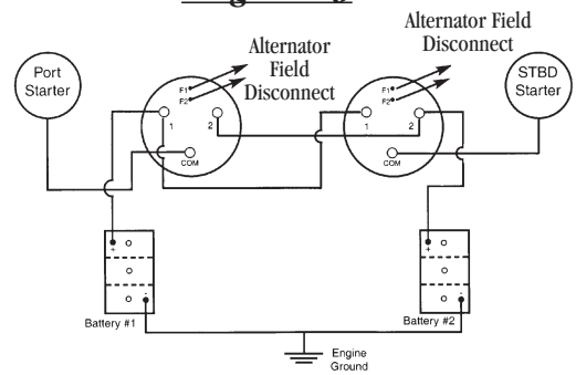
2 ENGINES, 2 BATTERIES, 2 SWITCHES.
