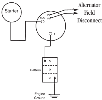
SINGLE ENGINE - SINGLE BATTERY
