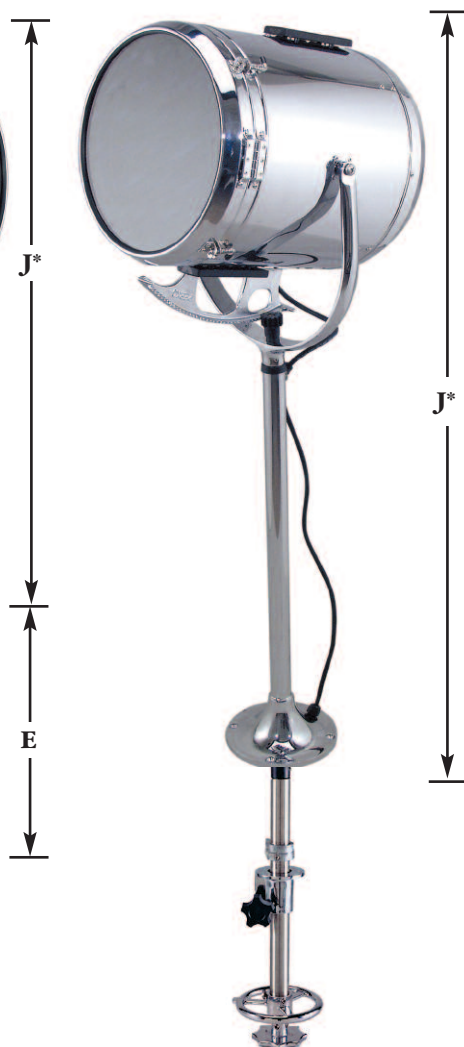
FIG. 885 HIGH PEDESTAL SHOWN WITH WHEEL CONTROL
