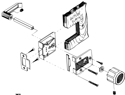
EXPLODED VIEW SHOWS FIG. 992
